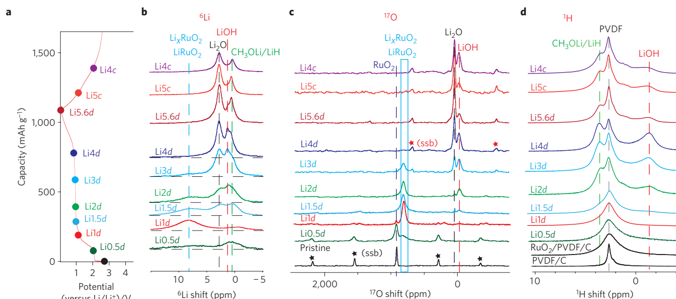
Figure 3 | Tracking the evolution of different chemical species at different states of charge in the \text{RuO}_2/\text{Li} battery system. a , The electrochemistry profile of \text{RuO}_2/\text{Li} cycled at a rate of C/48 . b–d , Ex situ ^6\text{Li} , ^{17}\text{O} and ^1\text{H} NMR spectra of DMC-washed samples cycled to various states of charge as marked on the electrochemistry profile. Dashed lines marking the baselines are shown for the first few spectra in the ^6\text{Li} series in b to assist in the observation of the broad \text{LiRuO}_2 peak at \sim 8 ppm. Asterisks in c indicate spinning side bands.
